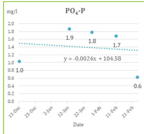
Graph 16 Average values of 22 sampling points for PO 4 -P
